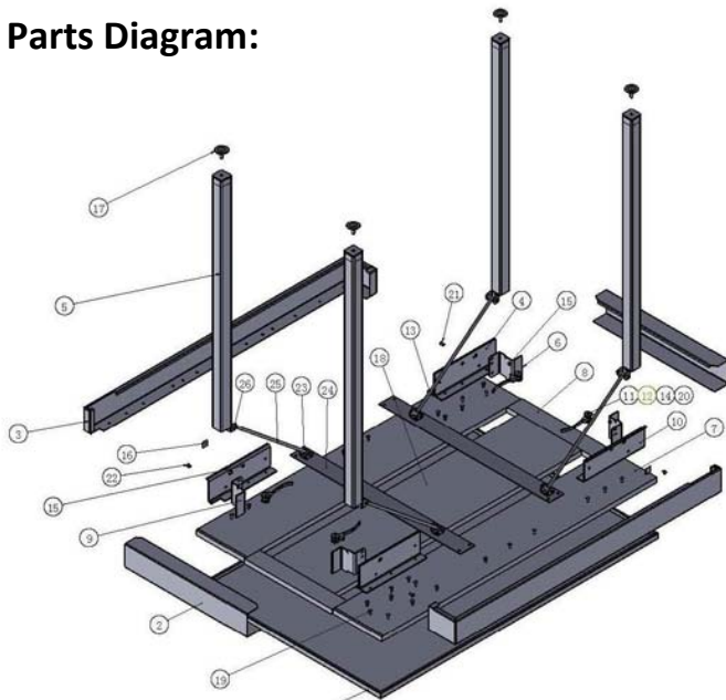
Folding Stainless Steel Processing Table
